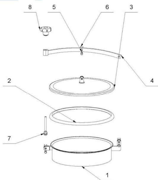
Exploded parts diagram
