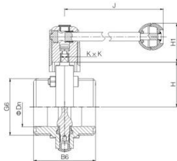
拉手柄蝶阀 Manual butterfly valve with pull handle NO.DS-VDF130S1
