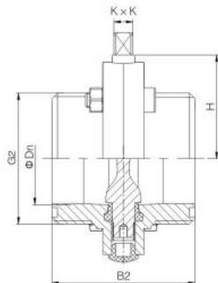
螺纹式MALE/MALE(SMS) NO.SMS-VDF130XX
