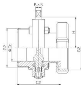
单螺纹单螺母式MALE/NUT(SMS) NO.SMS-VDF1Z0XX-23
