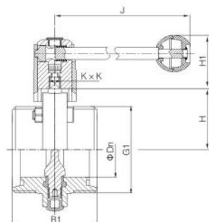
拉式手柄蝶阀 Manual butterfly valve NO.DIN-VDF130S1
