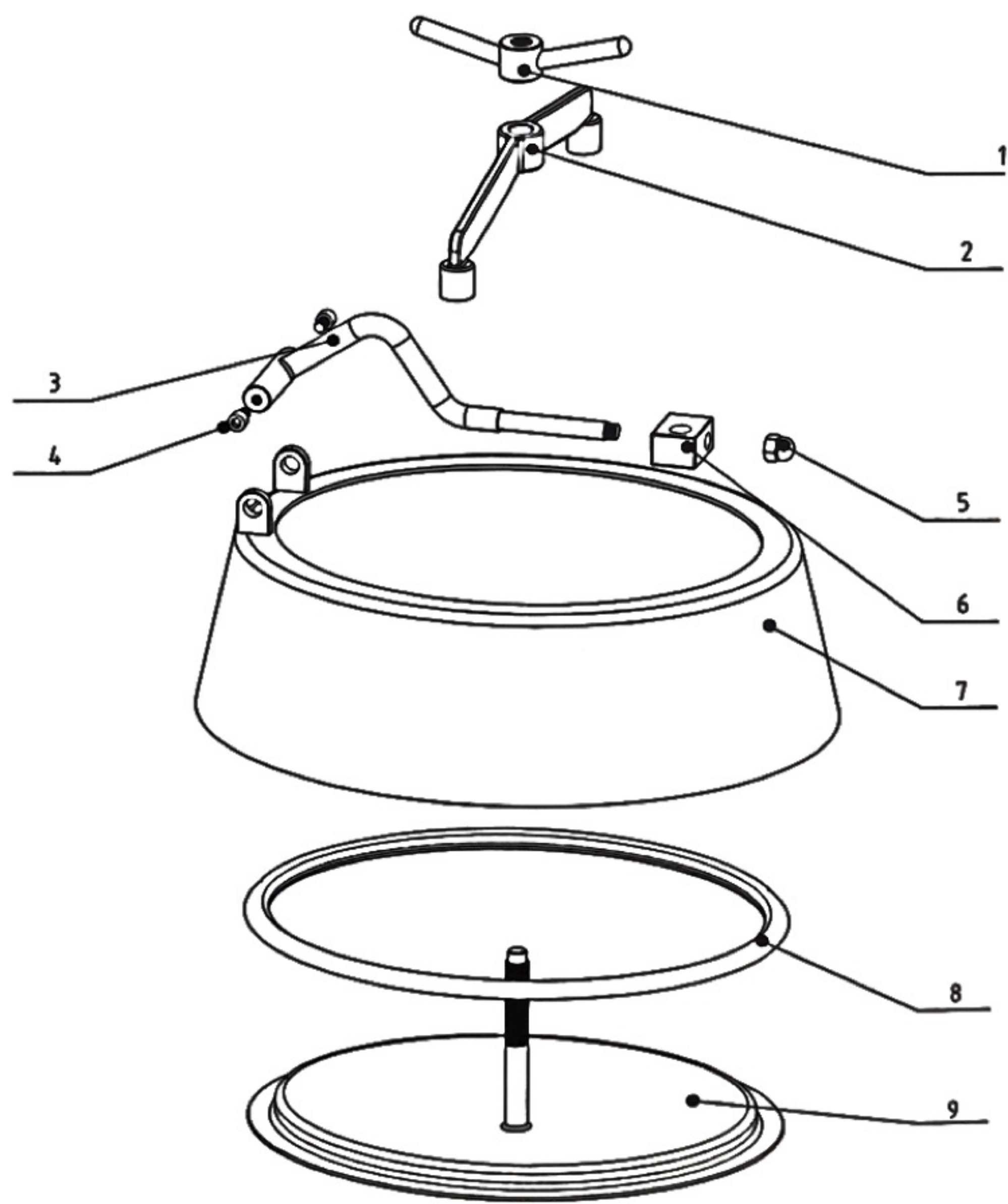
Exploded parts diagram
